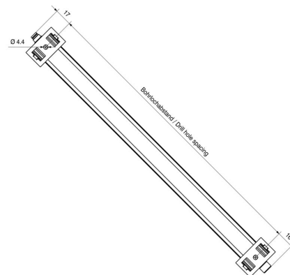
Dimensioned drawing
