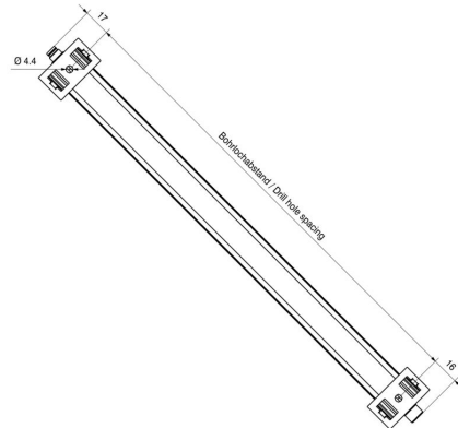
Dimensioned drawing
