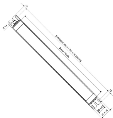
Dimensioned drawing
