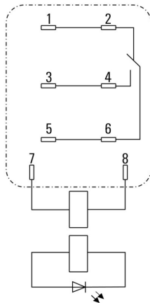
View of Pins from below
