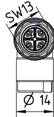
Dimensioned drawing
