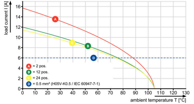
CPS 5.08/./270 - CH 5.08/./90G
