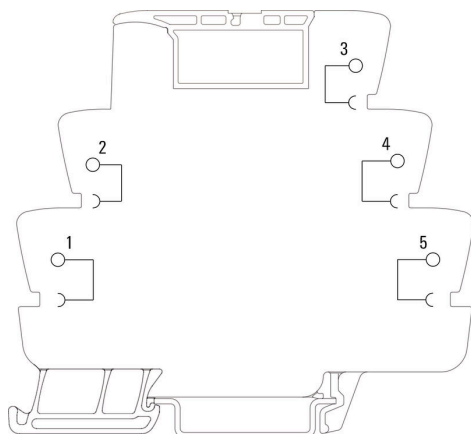
Wiring diagram
