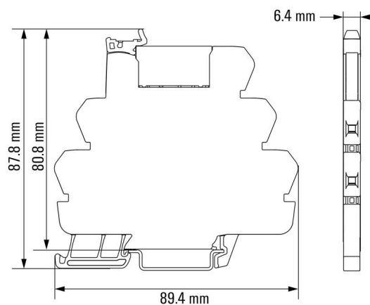
Dimensional drawing
