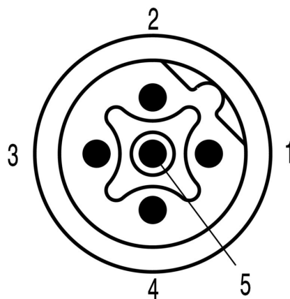
Pole scheme
