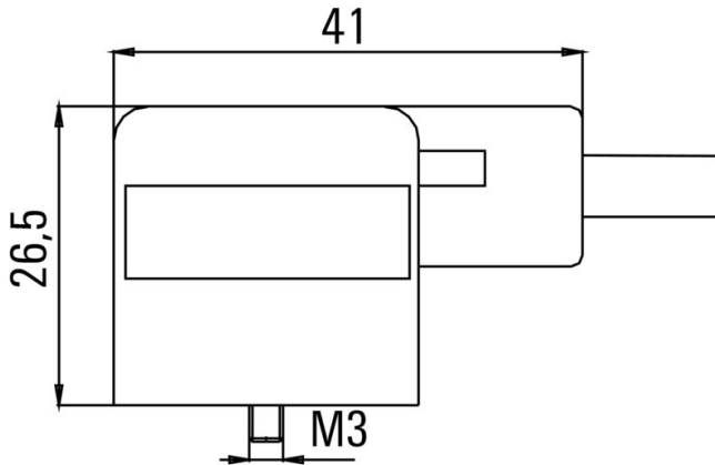
Dimensioned drawing
