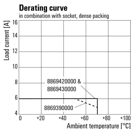
Derating curve
