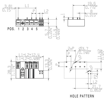
HOLE PATTERN
