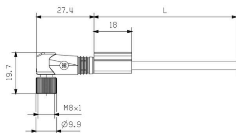
Angled socket
