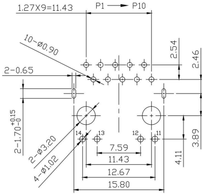
PCB LAYOUT 2
