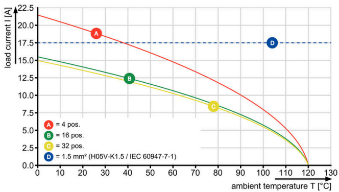
BCF 3.81/16/180 - SCDN-THR 3.81/16/90
