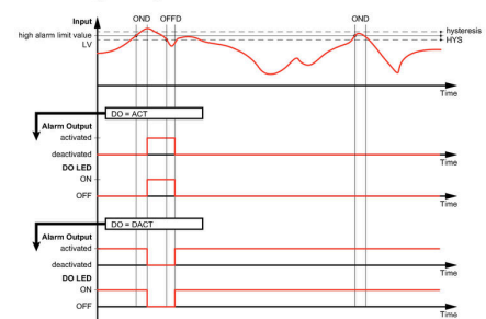
Measuring overrange
