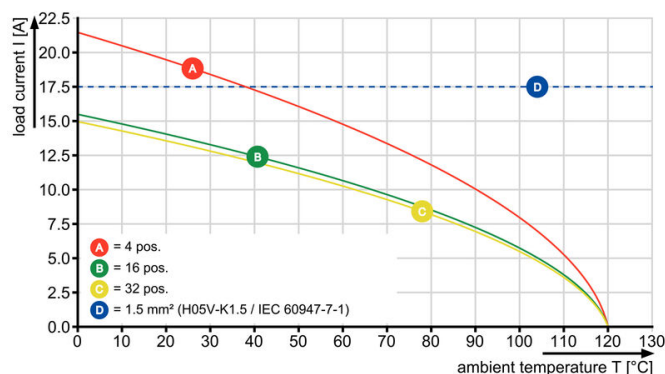
BCF 3.81/./180 - SCDN 3.81/./90
