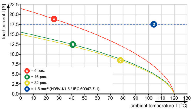
BCF 3.81/10/180 - SCDN-THR 3.81/10/90
