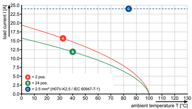
BLZP 5.08/.../225 - SL 5.08/.../90
