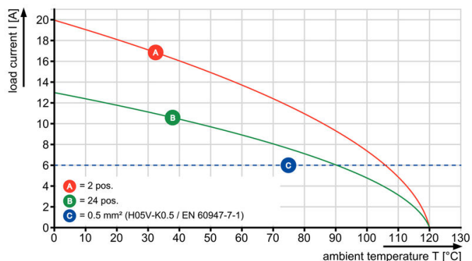
LSF-SMT 3.81/./135 1.5
