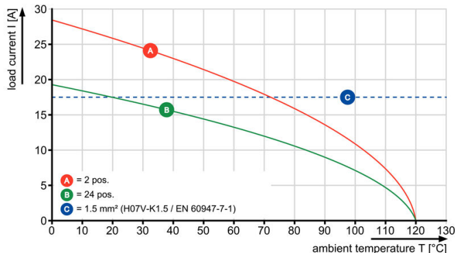
LSF-SMT 3.81/./135 1.5
