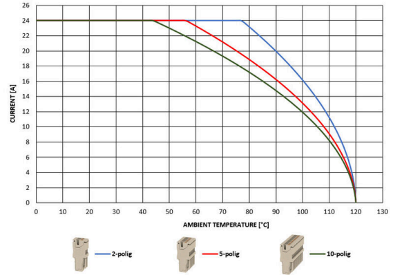
Derating APG 2.5...
