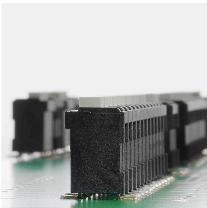
Stabile Lötanschlüsse
