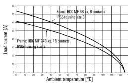
HDC-MHX 3-modules in the IP65-housing, Conductor H07V-K10:
