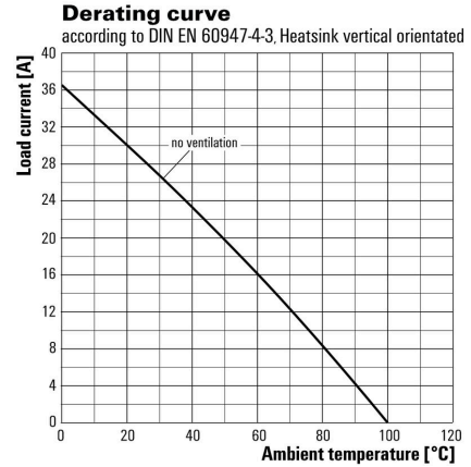
Deratingkurve
