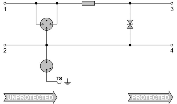
Circuit diagram
