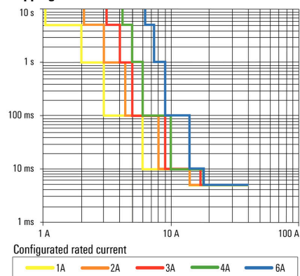
Tripping characteristic
