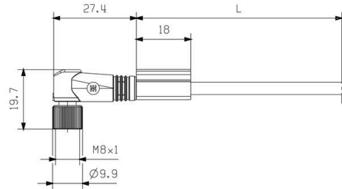
Angled socket
