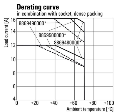
Relay in combination with base
