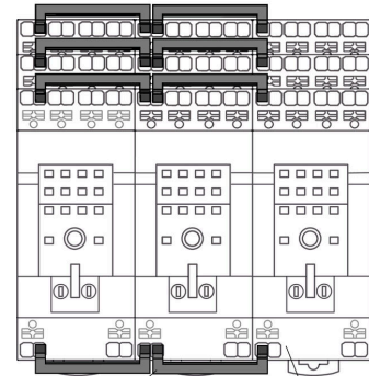
Sockets: for example CSM P 4CD Part-No. 3053140000
