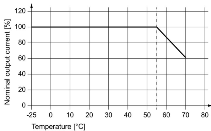
Temperature Derating
