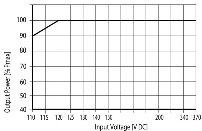
DC-Input Derating
