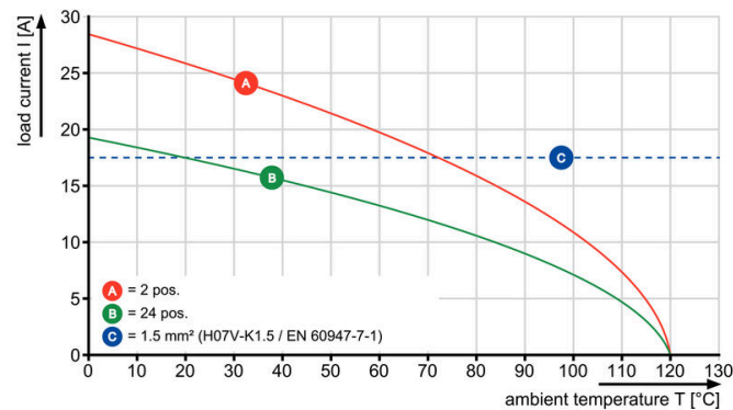
LSF-SMT 3.81/./135 1.5
