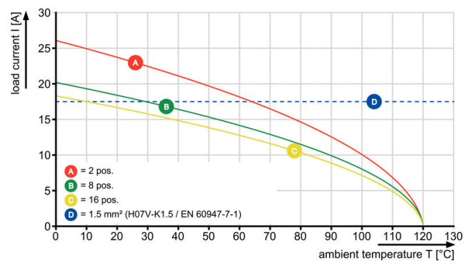
BCZ 3.81/./90 &amp; /270 - SC-SMT 3.81/./135
