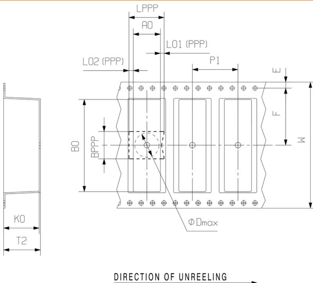
Packaged in tape-on-reel
