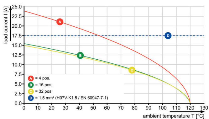
BCZ 3.81/./180 - SCDV 3.81/./90
