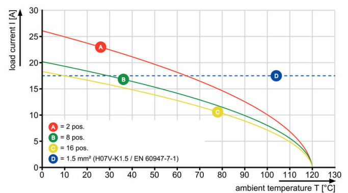
BCZ 3.81/./180 - SC-SMT 3.81/./135
