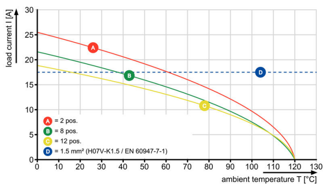
BCZ 3.81/./180 - SCZ 3.81/./180
