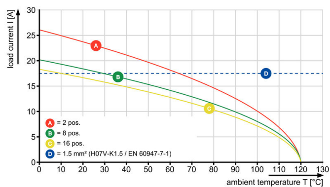
BCZ 3.81/./180 - SC-SMT 3.81/./135
